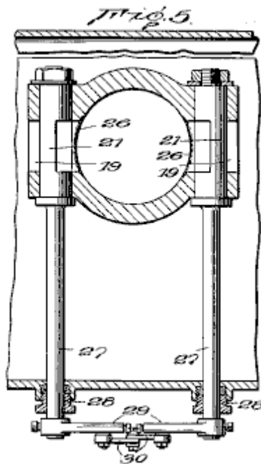
Fig.5 is a detail cross-sectional view showing the means for controlling the passage of gasses from the vapour expanding chamber into the intake manifold of the engine.
