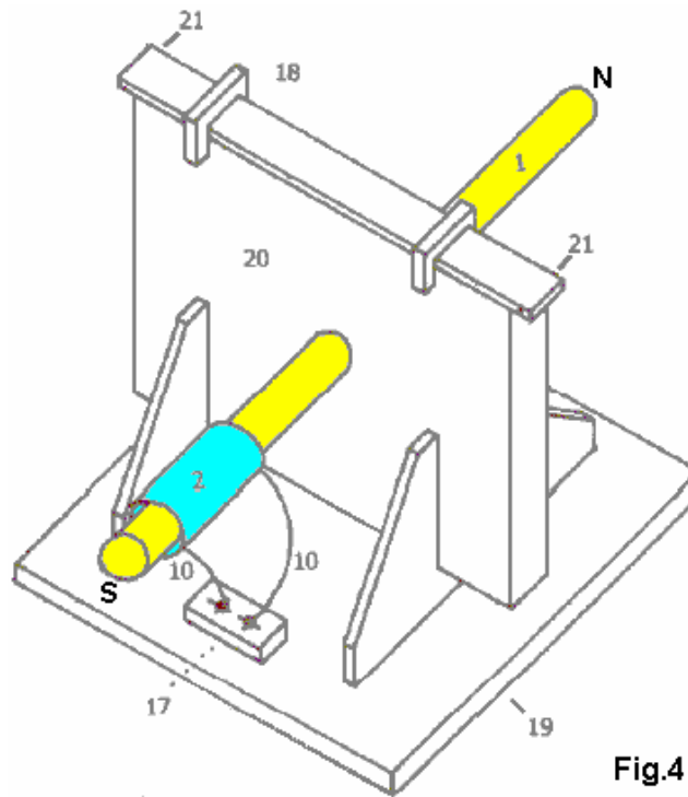
Fig.4 shows a Manufacturer's Prototype, constructed and fully tested. 1 is a metal Dipole rod and 2 the resonant high-voltage induction coil, connected through wires 10 to connector block 17 which facilitates the connection of it's high-voltage power supply. Clamps 18 hold the upper edge of the capacitor packet in place and 19 is the base plate with it's supporting brackets which hold the whole device in place. 20 is a housing which contains the capacitor plates and 21 is the point at which the power output from the capacitor plates is drawn off and fed to the DC inverter.
