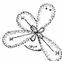
HYBRIDIZED AMMONIA MOLECULE NH_3
