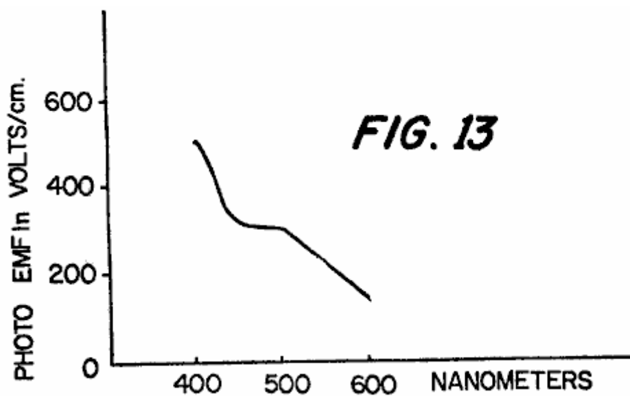
Fig.13 , is diagram illustrating the photo-emf vs. wave length of short wavelength cut-off filters, with the material being \text{Pb}(\text{Zr}_{0.53}\text{Ti}_{0.47})\text{O}_3 with 1% by weight of \text{Nb}_2\text{O}_5 added;
