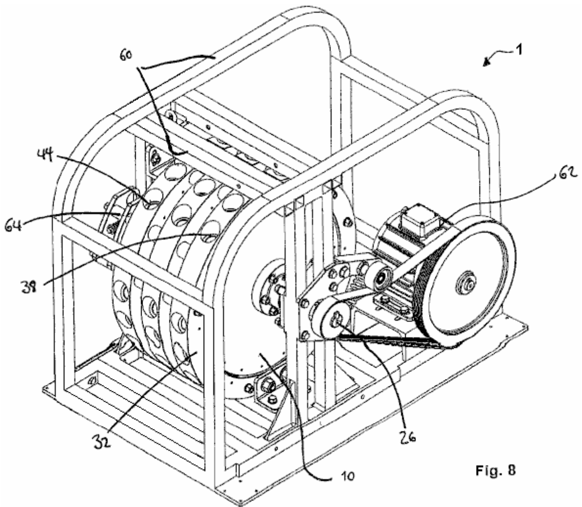
Fig.8 is a perspective view showing one embodiment of the magnetic repellent motor coupled to an electrical generator.
