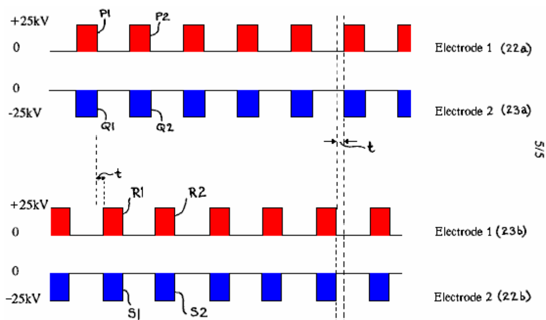
Fig.5 shows trains of pulses applied to electrodes of the fracture cell apparatus according to the invention.
